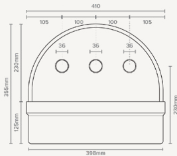
SECTION VIEW
