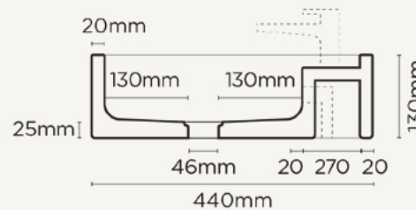
SECTION VIEW
