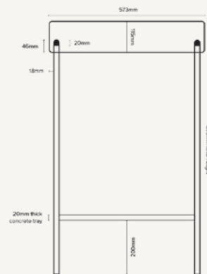
SECTION VIEW
